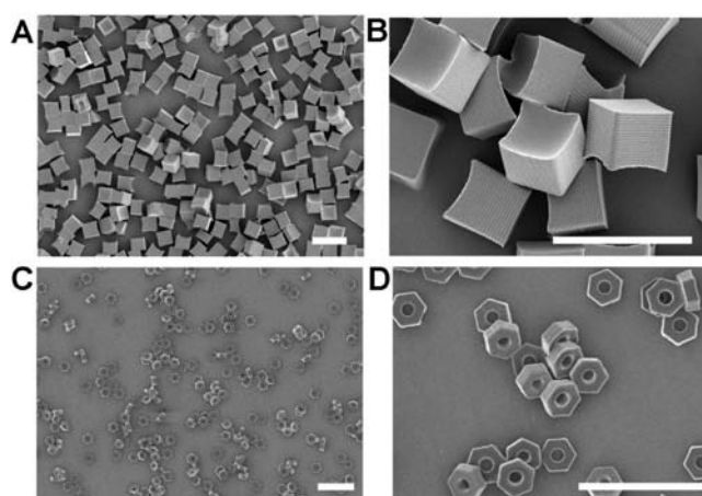
Figure 1. Scanning electron micrographs of (A, B) 5 μm cubes and (C, D) 3 μm hexnut particles fabricated using PRINT (scale bars: 10 μm).
